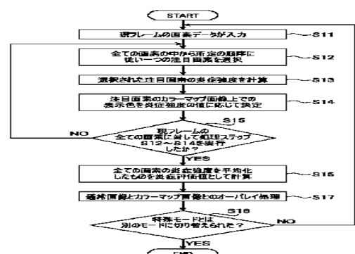
FIG. 2 S11 Input pixel data of current frame S12 Select one focus pixel from all pixels according to a prescribed selection S13 Calculate information severity for selected focus pixel S14 Determine display color of focus pixel on color map image according to information severity S15 Processing steps S12-S14 complete for all pixels of current frame? S16 Calculate information evaluation value as average of information severity of all pixels S17 Overlay normal image and color map image S18 Switched to a mode other than special mode?
